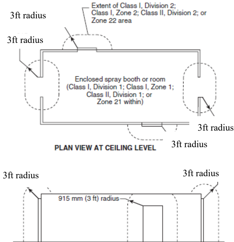
Figure 3 Class I, Division 2 Class I, Zone 2; Class II, Division 2; or Zone 22 Locations Adjacent to an Enclosed Spray Booth or Spray Room
