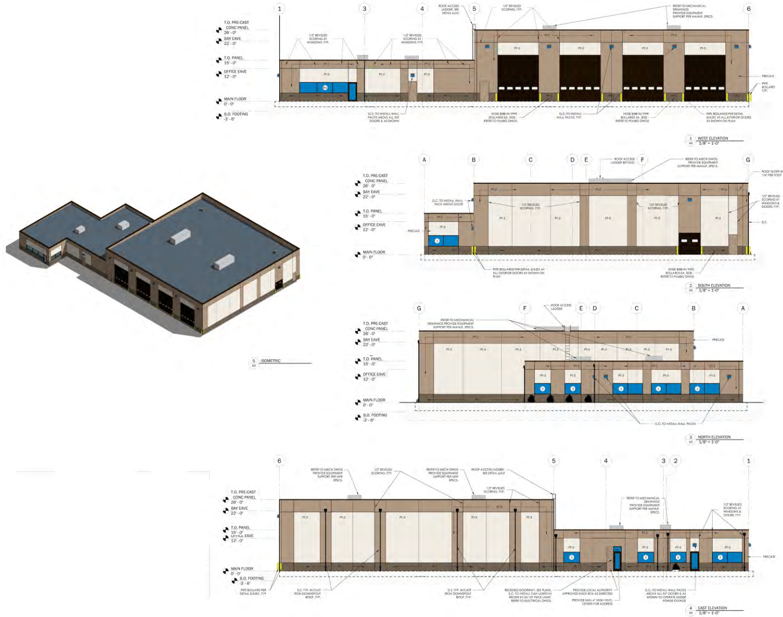
Figure 2.7-2 Building 2 Design
