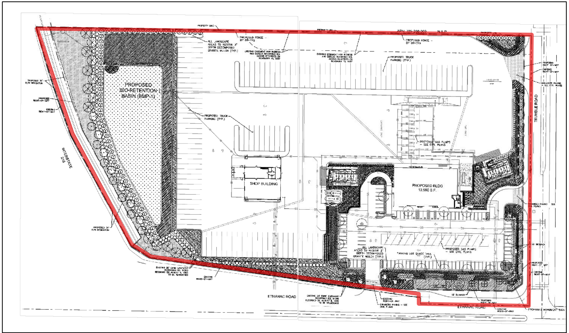
Figure 2-6. Preliminary Landscape Plan
