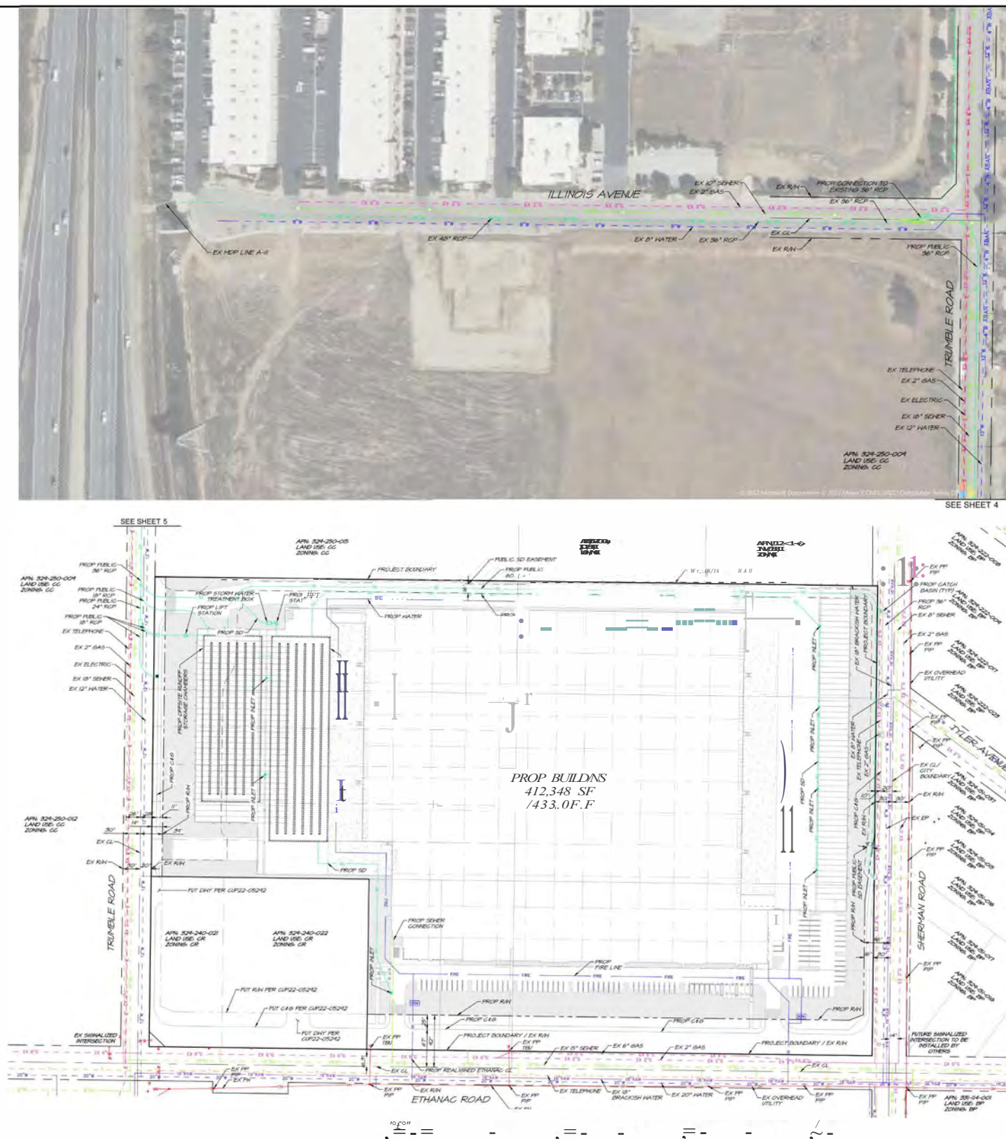
Figure 1.0-21 Existing and Proposed Conceptual Utilities (Alternative Option) Ethanac Logistics Center
