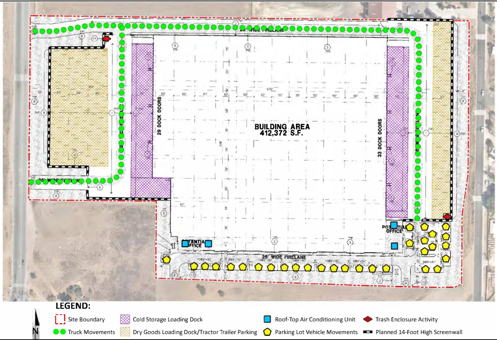
Figure 5.8-6 Operational Noise Source Locations Ethanac Logistics Center
