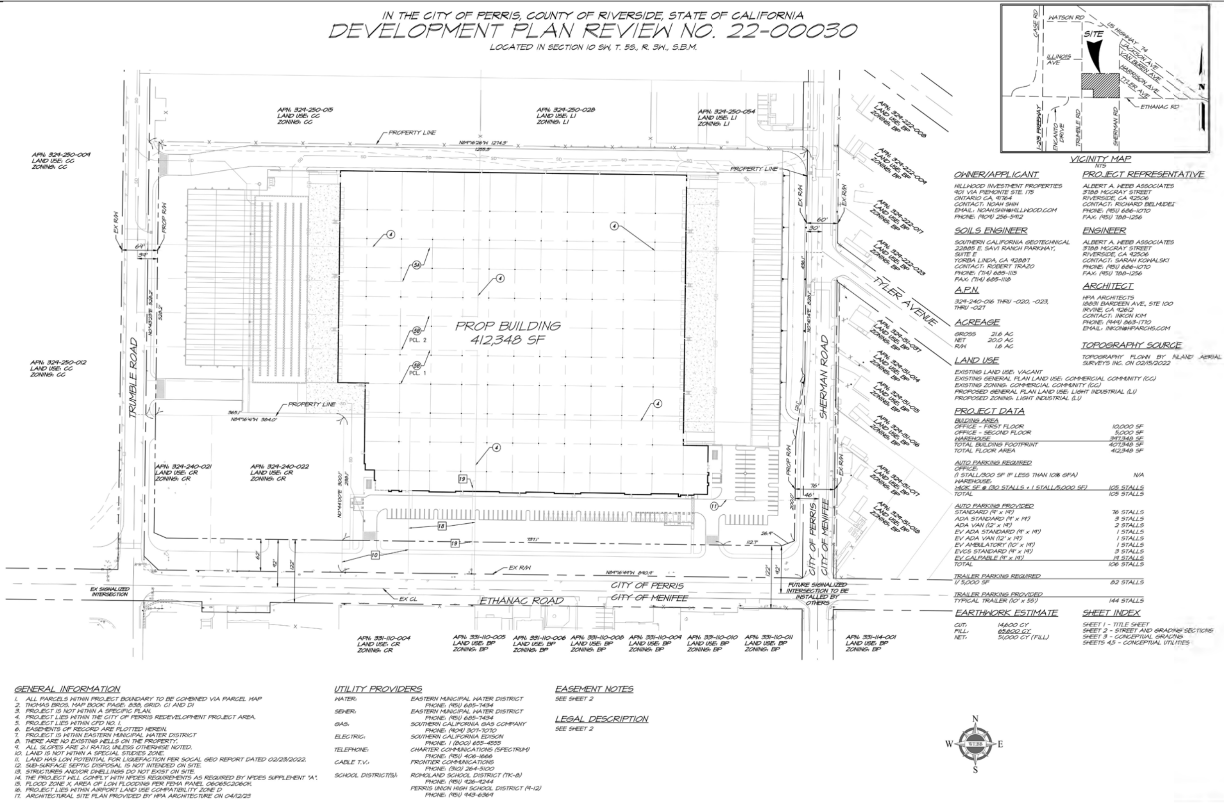
Figure 1.0-12 Development Plan Review Ethanac Logistics Center
