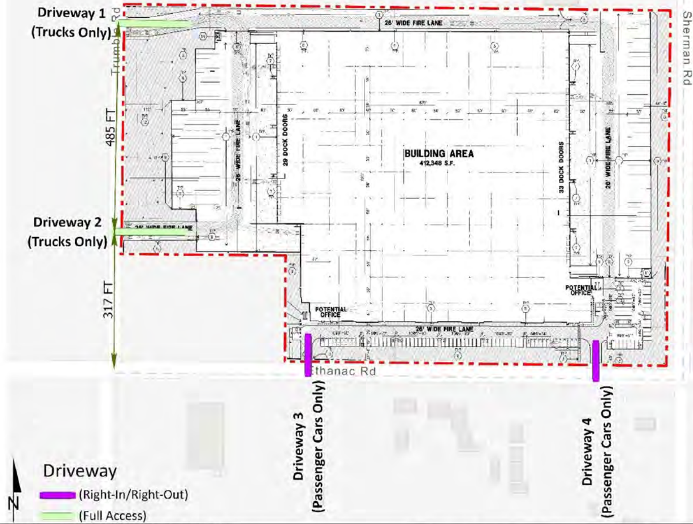
Figure 5.9-7 Proposed Project Site Driveways Ethanac Logistics Center
