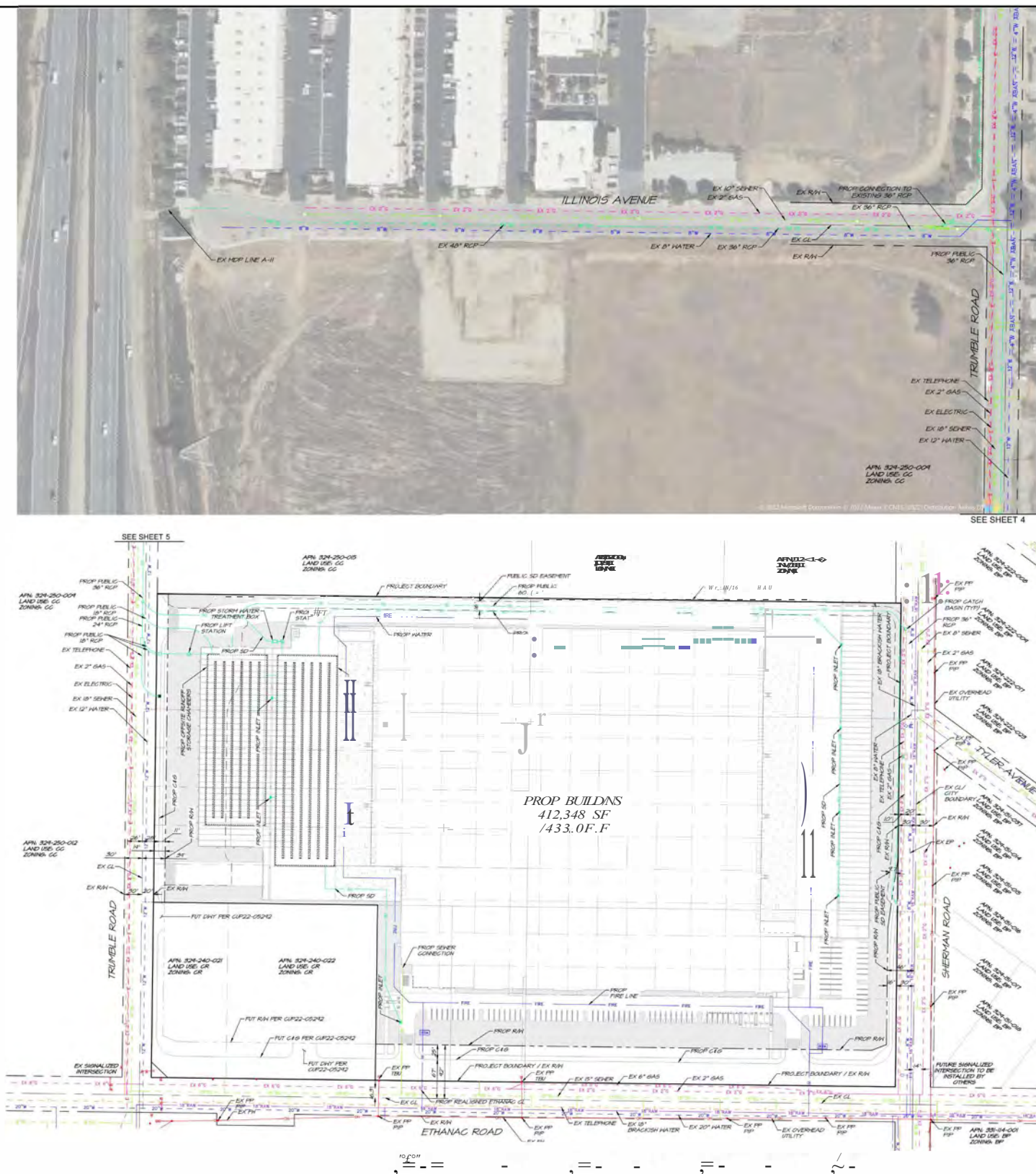
Figure 3.0-21 Existing and Proposed Conceptual Utilities (Alternative Option) Ethanac Logistics Center
