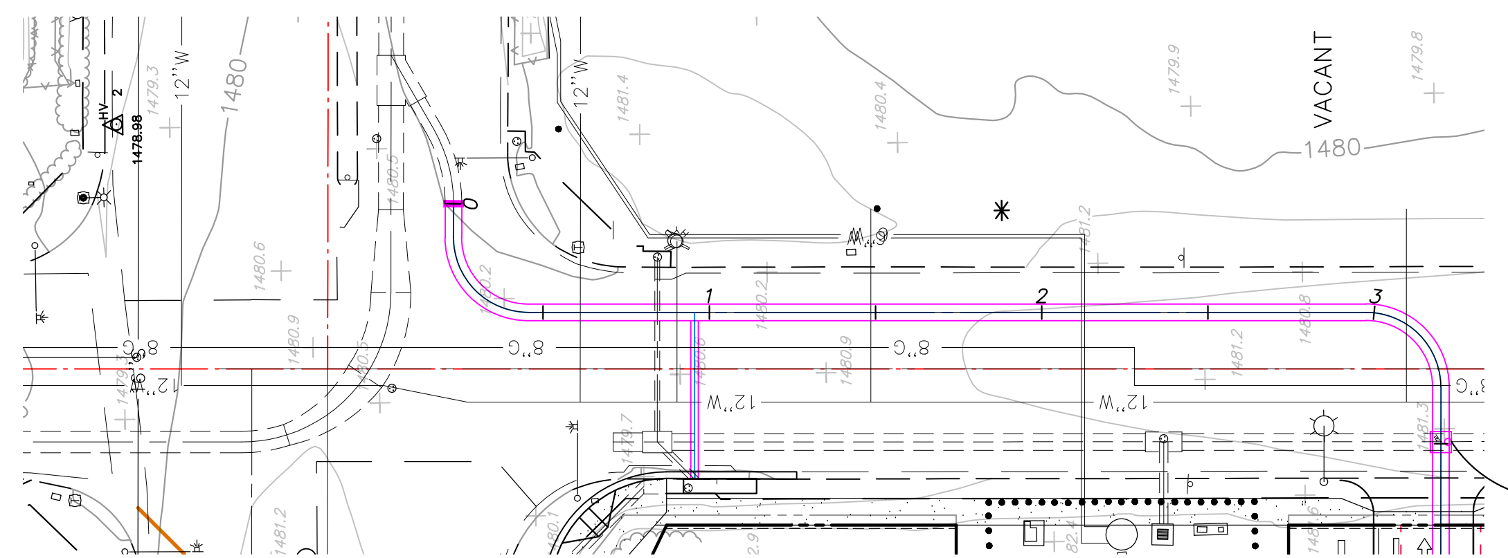
60" STORM DRAIN PLAN LINE 1
