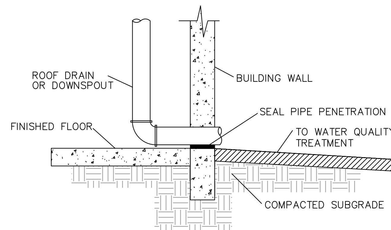
ROOF DRAIN DETAIL
