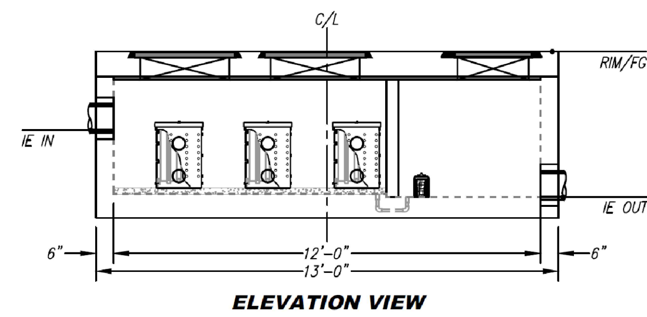
ELEVATION VIEW
