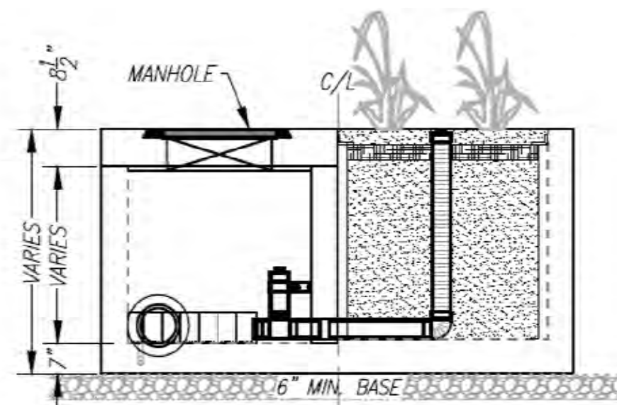
RIGHT END VIEW
