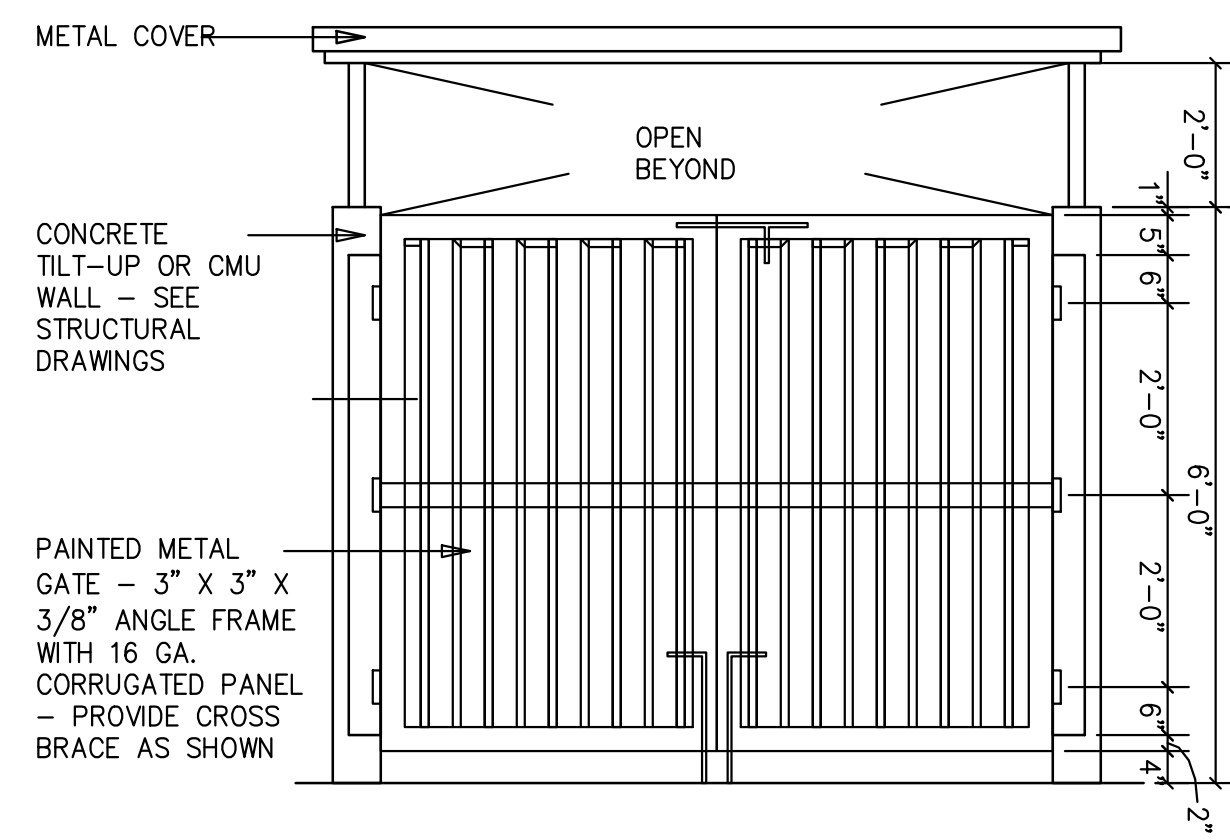
TYPICAL TRASH ENCLOSURE
