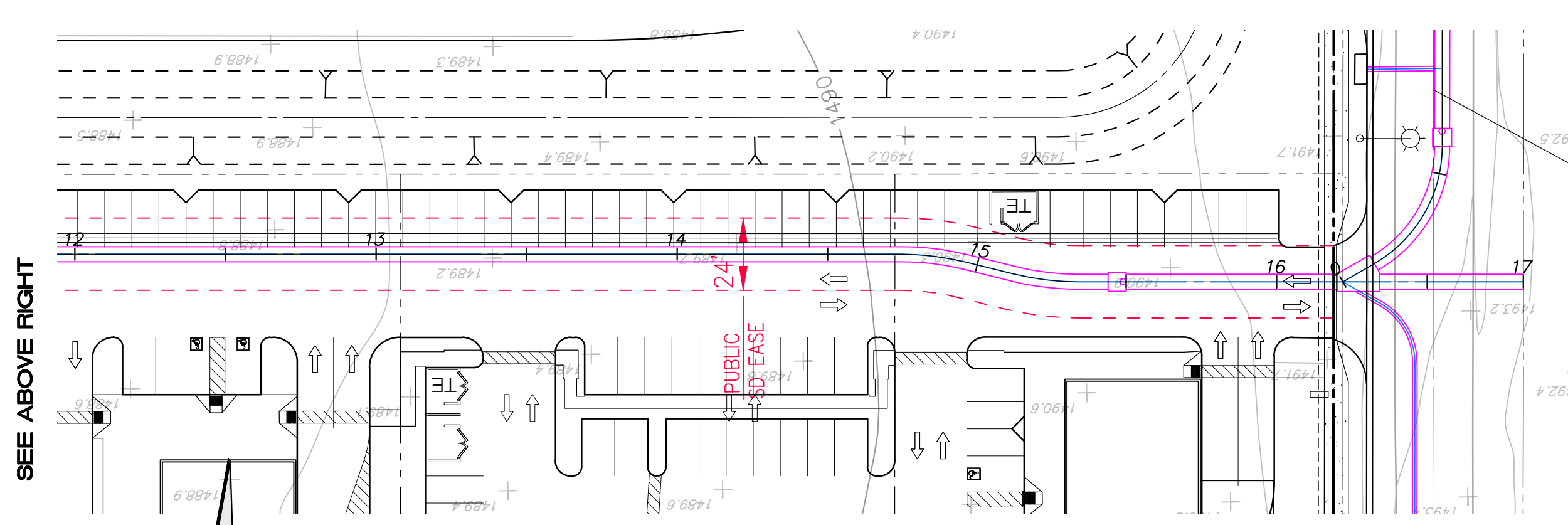
60" STORM DRAIN PLAN LINE 1
