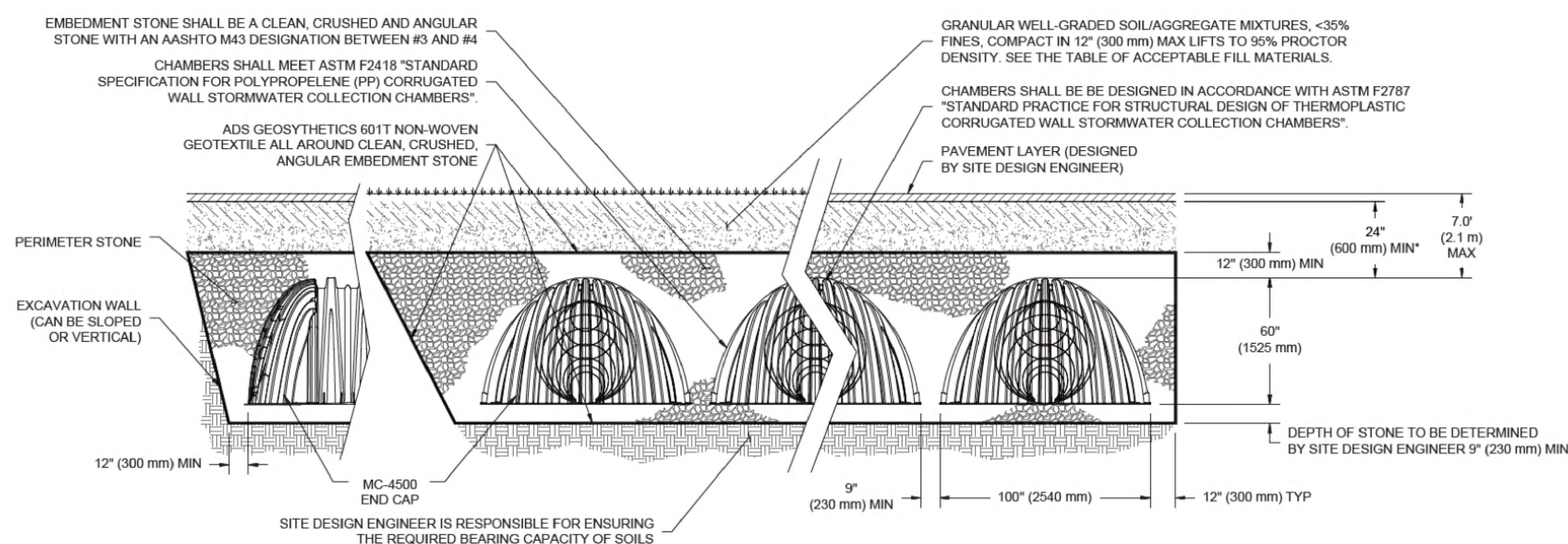
TYPICAL UNDERGROUND STORAGE SYSTEM
