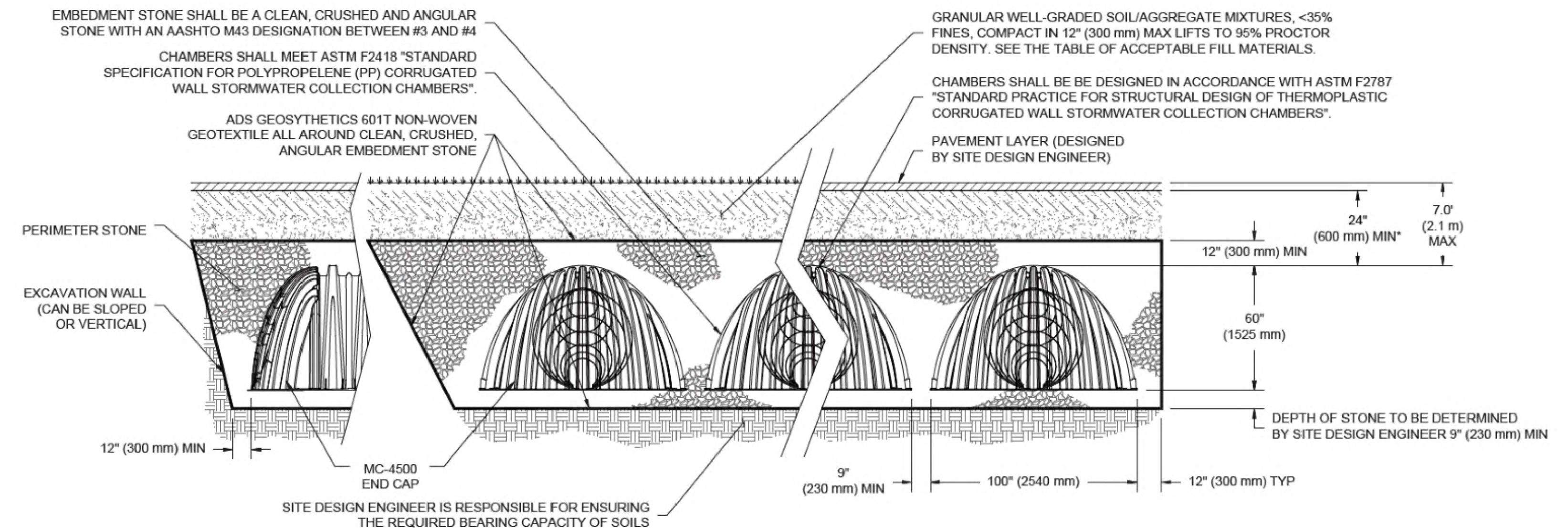
TYPICAL UNDERGROUND STORAGE SYSTEM
