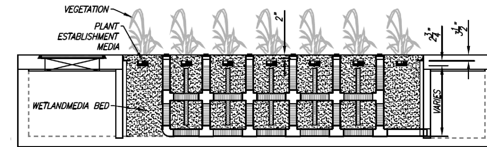
SECTION VIEW
