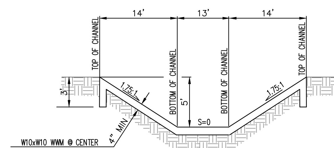
PROPOSED CONC CHANNEL N.T.S.
